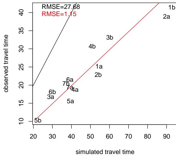
Figure 5: Calibration of the travel times. The solid black line is the y = x diagonal; the red line is y = e^{-0.70}x , corresponding to the calibration in equation (6). The corresponding root mean square error (RMSE) is given in the legend. The points are numbered according to the routes in Figure 4.
